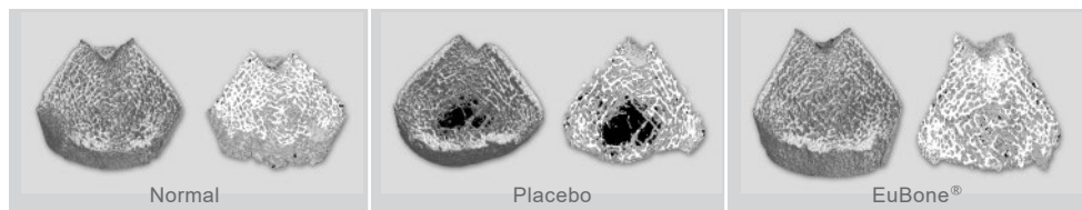
3D-microCT images
